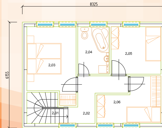
poschodie
