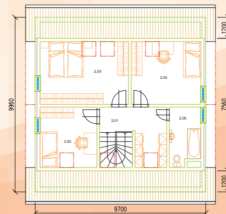
poschodie
