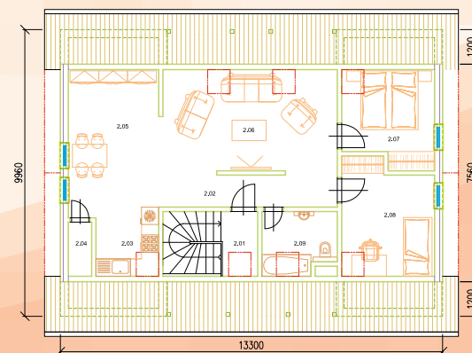
poschodie
